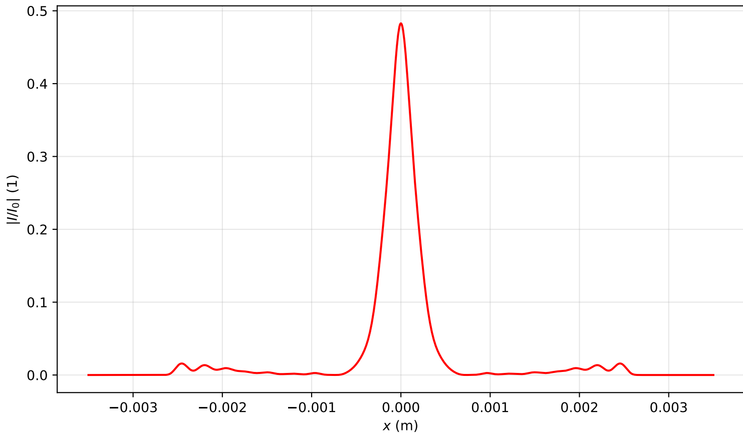
Intensity profile I(x, y = 0, z = 1.751)/I_0 , P_{in}=6.0P_{cr} , artificial time
